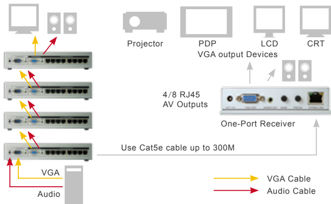
Stack Four 8-Port System Transceiver Locally to Generate More RJ-45 AV Output Signals
