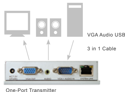
Installation Diagram of System Transmitter AVE-301T
