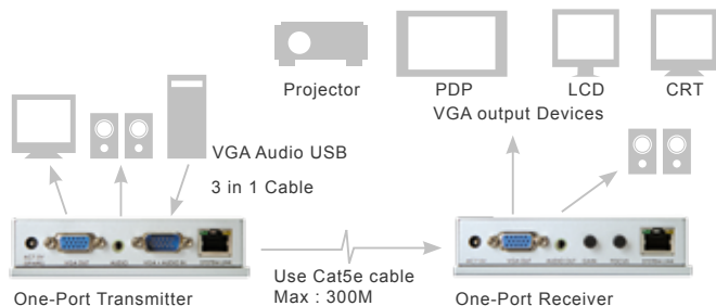
Installation Diagram of Receiver AVE-301R
