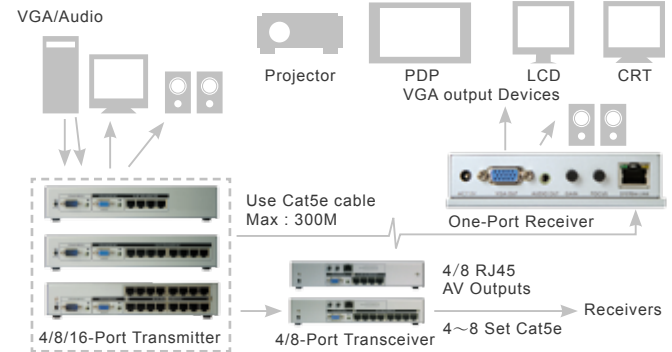
Installation Diagram of System Receiver and Trans
