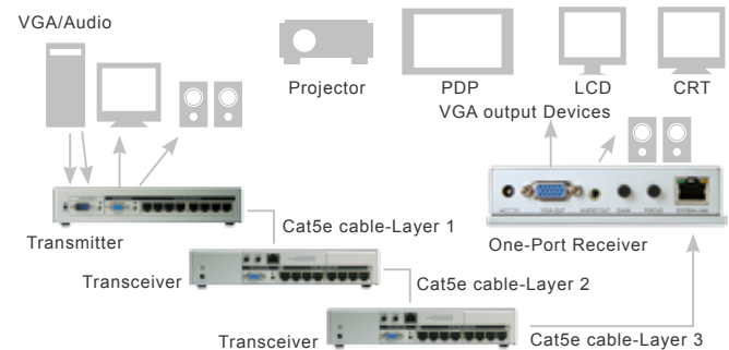
Stack Three Layers of AV Extender through Cat5e to Reach more Displays
